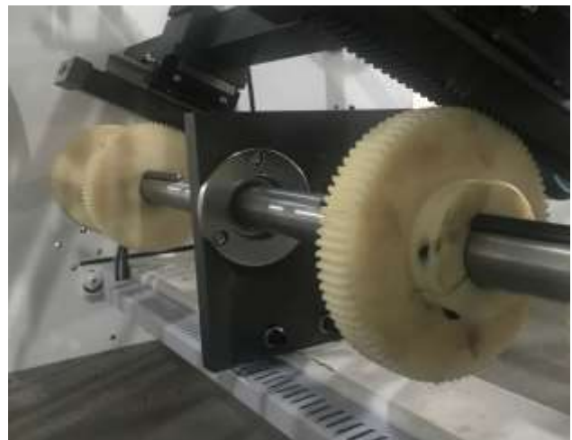
➤ Motor controlled gluing system. Inject glue and change the gluing sponge easily and quickly.
